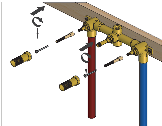
Install volume stem extension kit, tighten screws and then install longer trim piece
