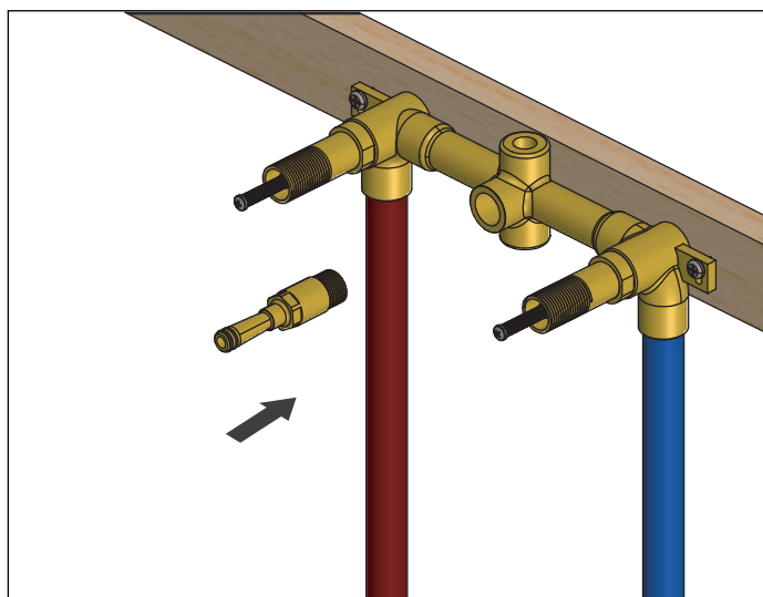
Insert longer spout extension piece
