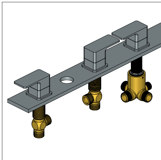
Install handle base and tighten set-screw
